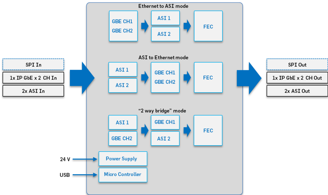
Block diagram ASI to IP converter 2 ways
